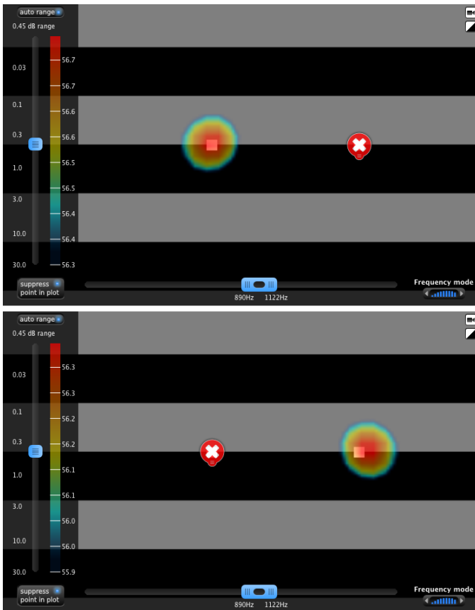
Fig. 15. Using the acoustic eraser to discover two perfectly coherent sources
